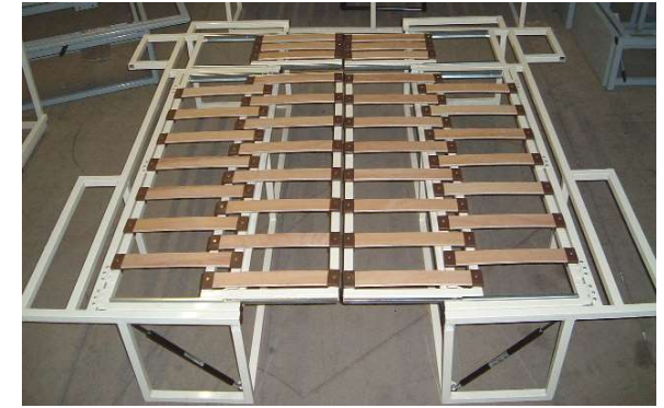
Configuration 3 – large double bed 1740mm long x 1720m wide
